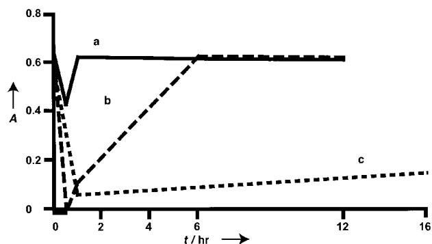
Figure 3. Change in the intensity of the ferrocenium absorption band (618 nm) upon UV illumination for 30 min (marked by bar along abscissa) followed by the bubbling of gases through the \text{TiO}_2 suspension in darkness (see text). a) —: \text{O}_2 ; b) ---: air; c) ----: \text{N}_2 .
