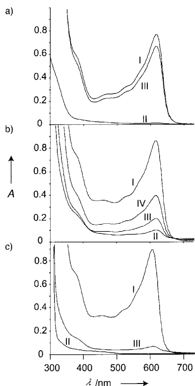
Figure 2. UV/Vis absorption spectra of supernatant solutions from suspensions of ODS- \text{TiO}_2 showing the redox-switching of ferrocene/ferrocenium ( \text{Fc}/\text{Fc}^+ ); initial [\text{Fc}^+\text{BF}_4^-] = 2 \text{ mM} . a) 1M HCl solution in ethanol. I: Initial \text{Fc}^+ solution; II: after UV-irradiation for 25 min; III: after stirring in the dark for 14 h. b) 0.1M HCl solution in ethanol. I: Initial \text{Fc}^+ solution; II: after UV-irradiation for 60 min; III: after stirring in the dark for 40 h; IV: after stirring in the dark for 70 h. c) 0.01M \text{HBF}_4 solution in ethanol. I: Initial \text{Fc}^+ solution; II: after UV-irradiation for 40 min; III: after stirring in the dark overnight (ca. 14 h).
